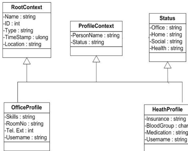
Figure 4. XML Schema
