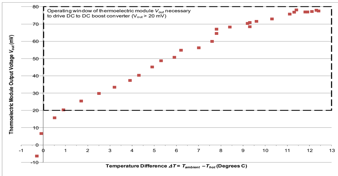
Figure 4. Thermoelectric module output voltage V_{out} with a temperature difference \Delta T of between 0^\circ\text{C} to 13^\circ\text{C} below ambient of 22^\circ\text{C} using a 71-couple 30mm x 30mm x 3.8mm thermoelectric module.
