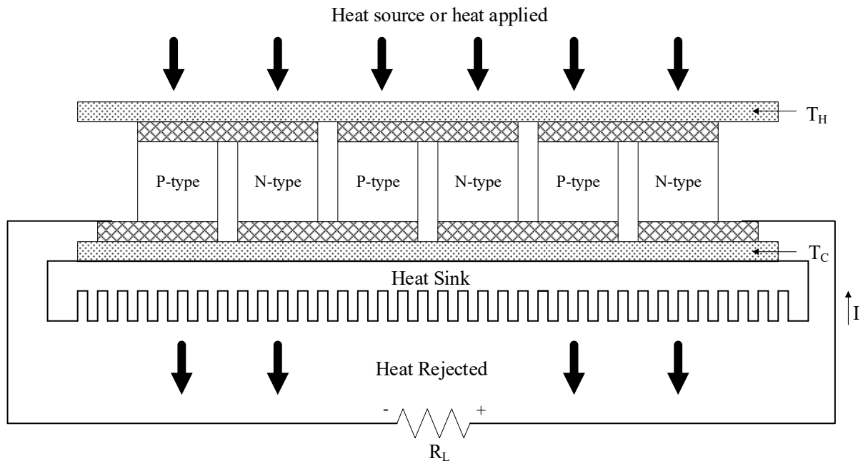
Figure 1. A thermoelectric module configured to operate as a thermoelectric generator [10].
