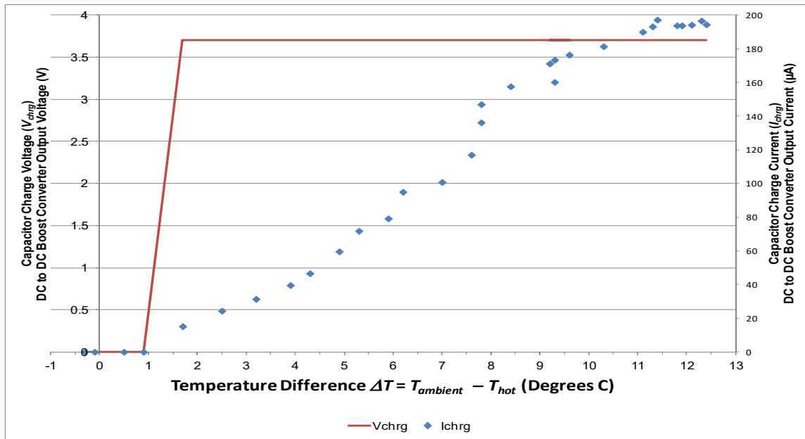
Figure 5. The capacitor charge voltage and current (DC to DC boost converter output voltage and current) V_{chrg} and I_{chrg} with a temperature difference \Delta T of between 0^{\circ}\text{C} to 13^{\circ}\text{C} below ambient of 22^{\circ}\text{C} using a 71-couple 30\text{mm} \times 30\text{mm} \times 3.8\text{mm} thermoelectric module.
