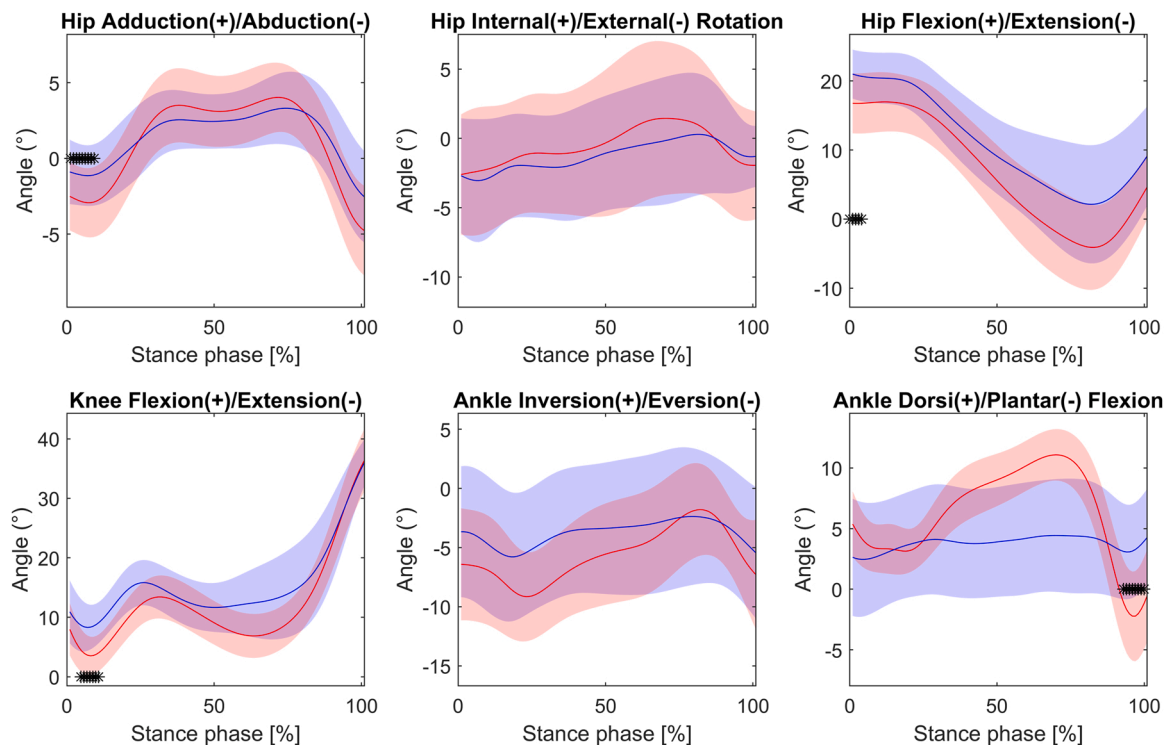
Fig. 3. Joint angles during the stance phase. The mean ( ± one standard deviation) values of the kinematic variables for NoTCC are illustrated in red while with blue the respective values for the trials performed with TCC. Significant differences ( p < 0.01 ) are denoted with ‘*’ on the x axis.
