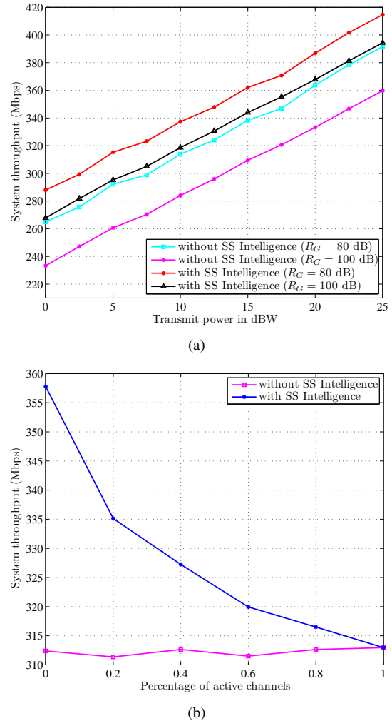
Fig. 3: (a) System throughput versus BS transmit power, (b) System throughput versus percentage of the active channels (BS transmit power P_{t,BS} = 10 dBW, R_G = 100 dB)
