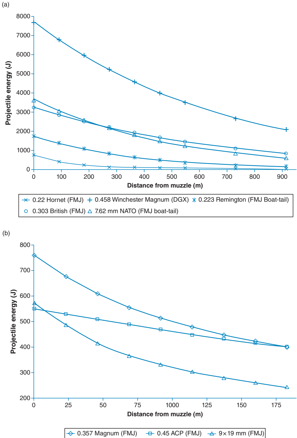
Fig. 7.1.2. Projectile energy changes for some common cartridges.
