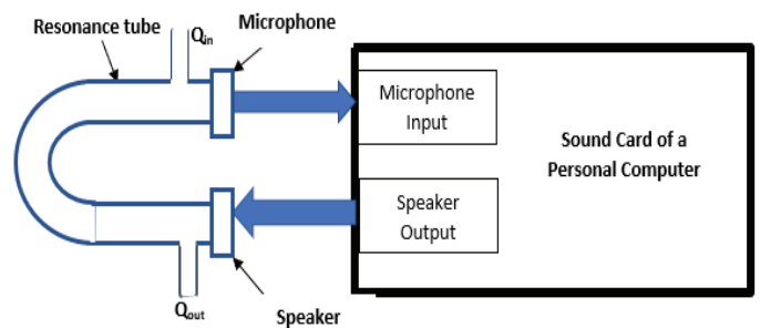
Figure 1. The schematic design of acoustic resonance detector for determination of the ratio C_p / C_v
