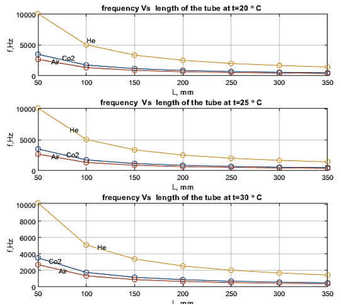
Figure 3. The plot(s) between the frequency of standing wave and the length of the tube at different temperature points
