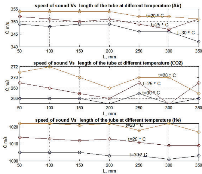
Figure 4. The variation of speed of sound vs. the length of the tube (at different temperature points)
