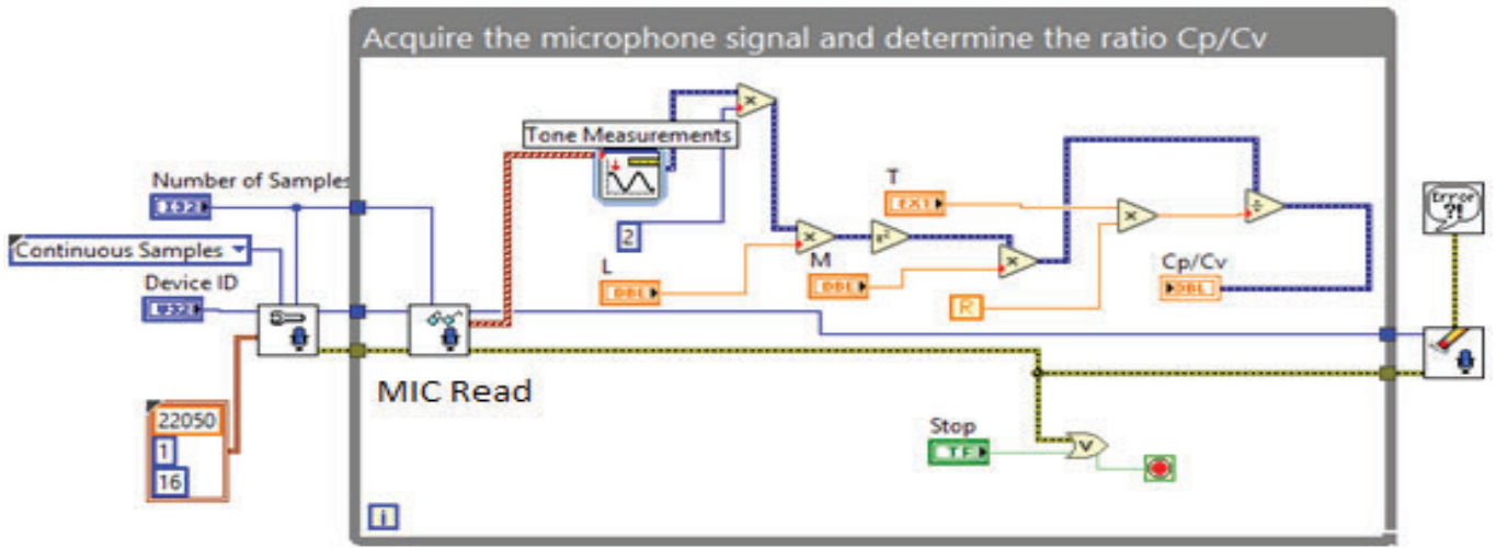
Figure 2. The VI design to acquire the microphone signal and determine the ratio C_p/C_v
