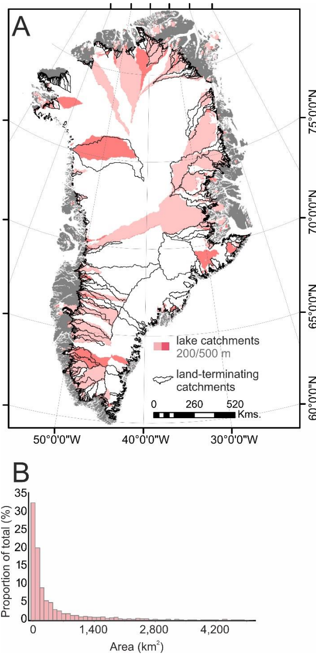
Figure 3. Catchment areas of ice-marginal lakes (A), where darker shades denote usage of a more lenient parameterisation and each is in addition to the area estimated with the lower leniency. Land-terminating catchments in panel A are from Mankoff et al. (2019b). Histogram analysis of the areal extent of the catchment areas highlights predominance of smaller lake catchments (B).
