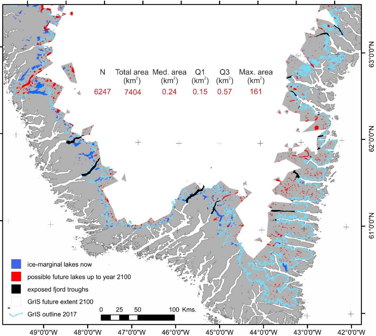
Figure 4. Location, number and size of overdeepenings, within which lakes could form in the future. Future 2100 ice extent is the mean of several models at 5 km resolution evaluated and reported by Goelzer et al. (2020). Inset statistics are for the whole of the GrIS, not just the southern part, which is depicted here to highlight the spatial differences. Note that the possible future lakes are a maximum estimate because not all will be ice-marginal simultaneously; many will become detached from the ice margin, and because we cannot suggest if all overdeepenings will completely fill with meltwater and not drain.
