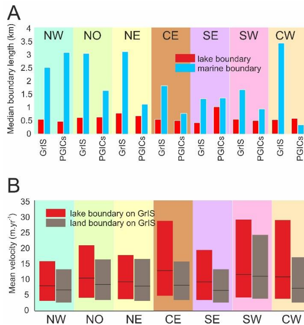
Figure 2. Comparison of boundary length (A) and mean velocity with boundary type (B) discriminated by region both for the GrIS and for PGICs. Inter-quartile range and maximum lake sizes are not displayed for clarity in panel A. The inter-quartile range and median are represented in panel B by a bar and a horizontal line, respectively.
