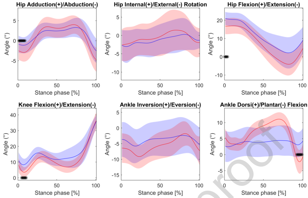
Figure 3: Joint angles during the stance phase. The mean ( \pm one standard deviation) values of the kinematic variables for NoTCC are illustrated in red while with blue the respective values for the trials performed with TCC. Significant differences ( p < 0.01 ) are denoted with '*' on the x axis.
