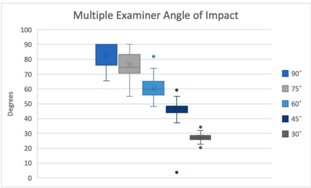
Fig. 5. Multiple examiners (10) determinations of the angle of impact showing the mean (x), range (line bar), and standard deviation (color bar) at five known angles for 10 stains at each known angle.
